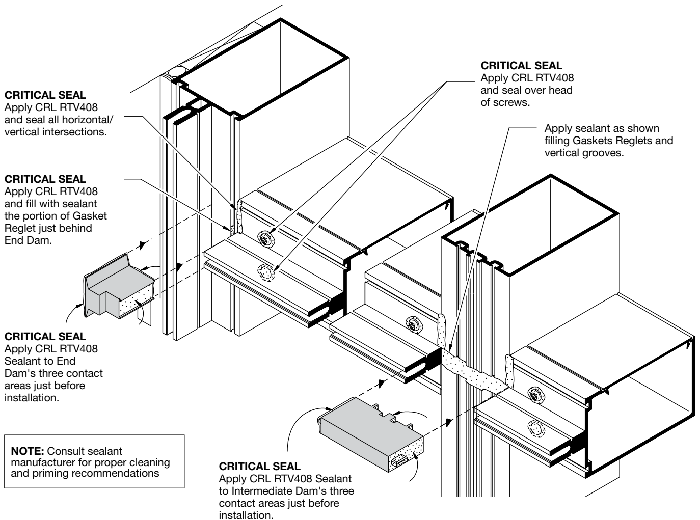
DETAIL P
