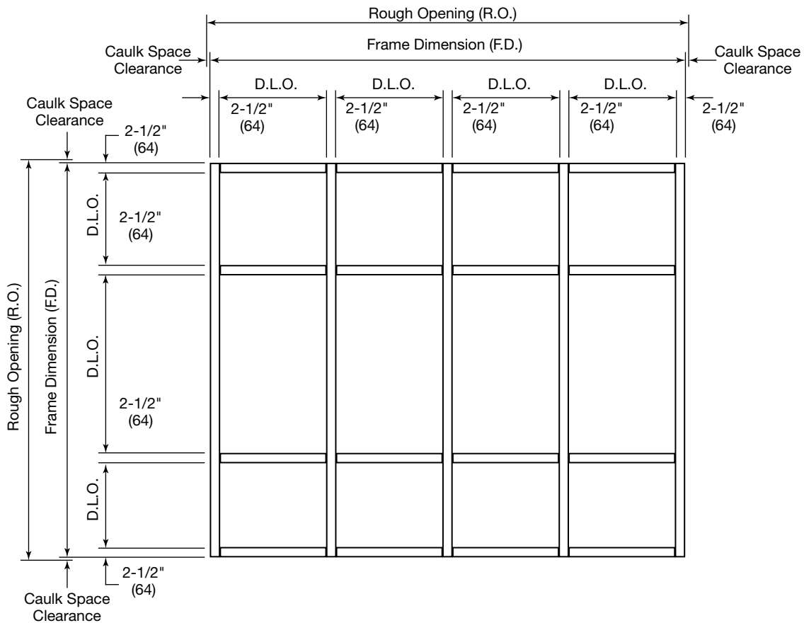
TYPICAL ELEVATION
