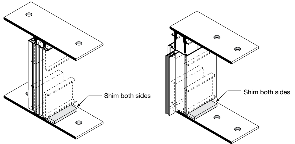
DETAIL F
