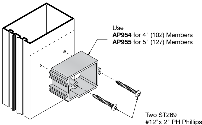
DETAIL G
