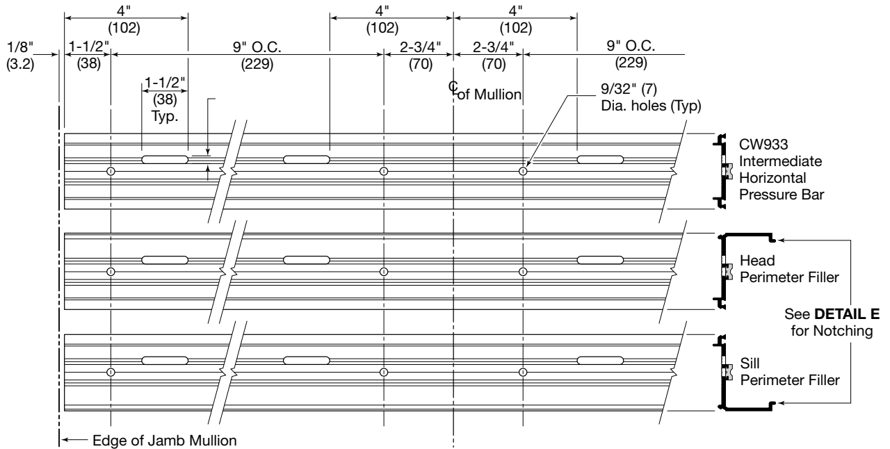
DETAIL D
