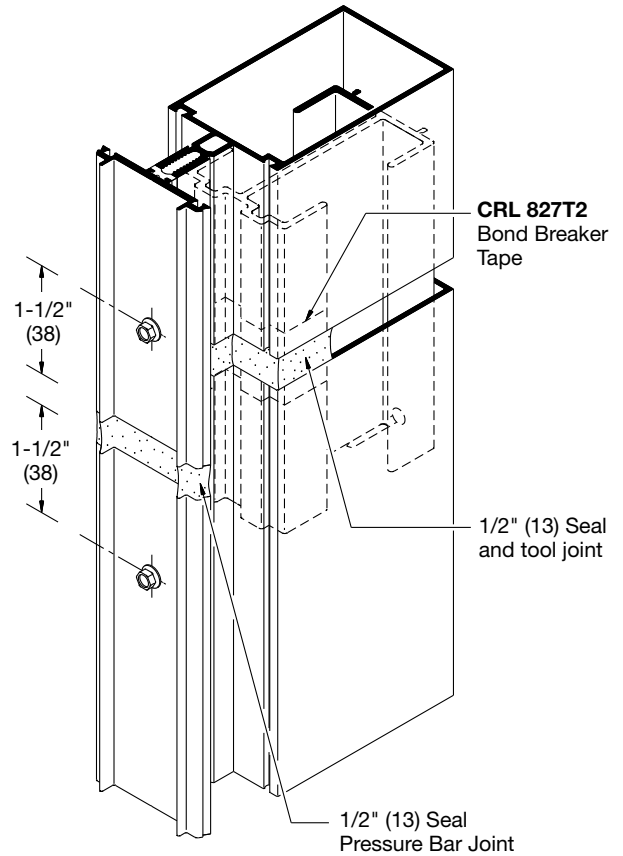
DETAIL CC
