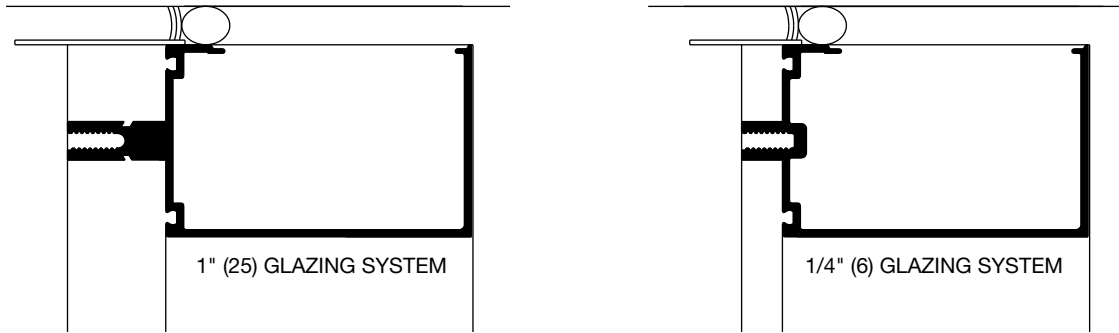
DETAIL O
