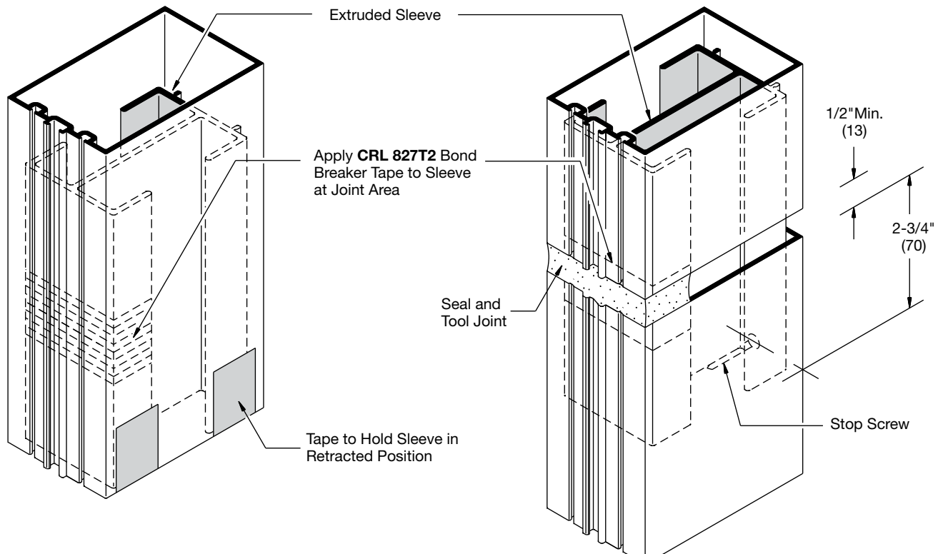
DETAIL AA
