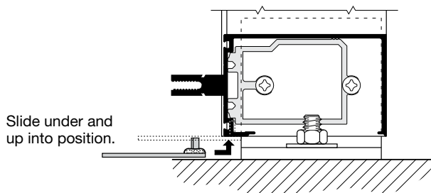
DETAIL N
