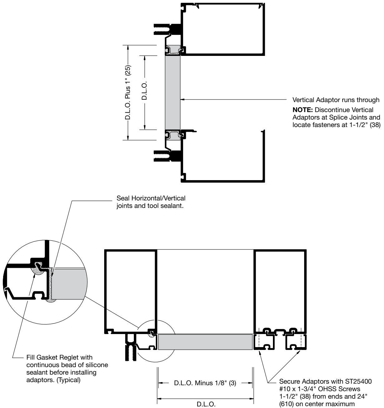
DETAIL Z
