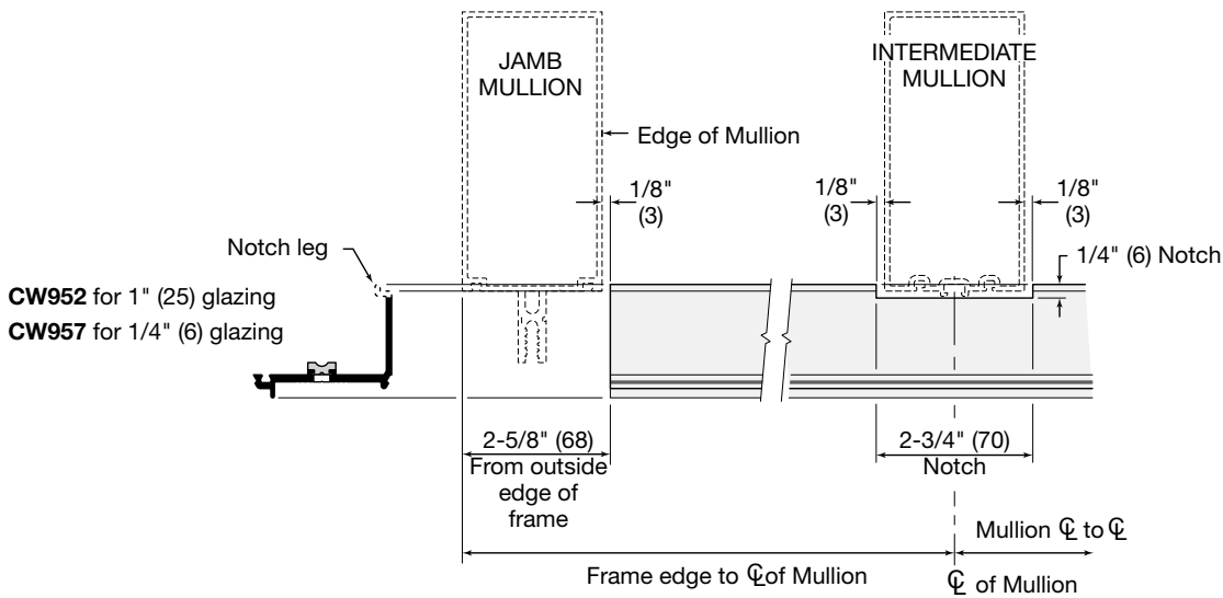
DETAIL E
