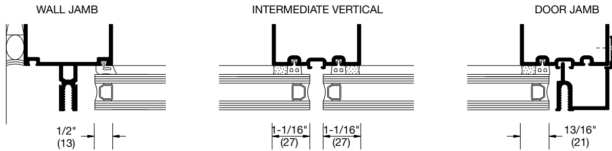
DETAIL Q
