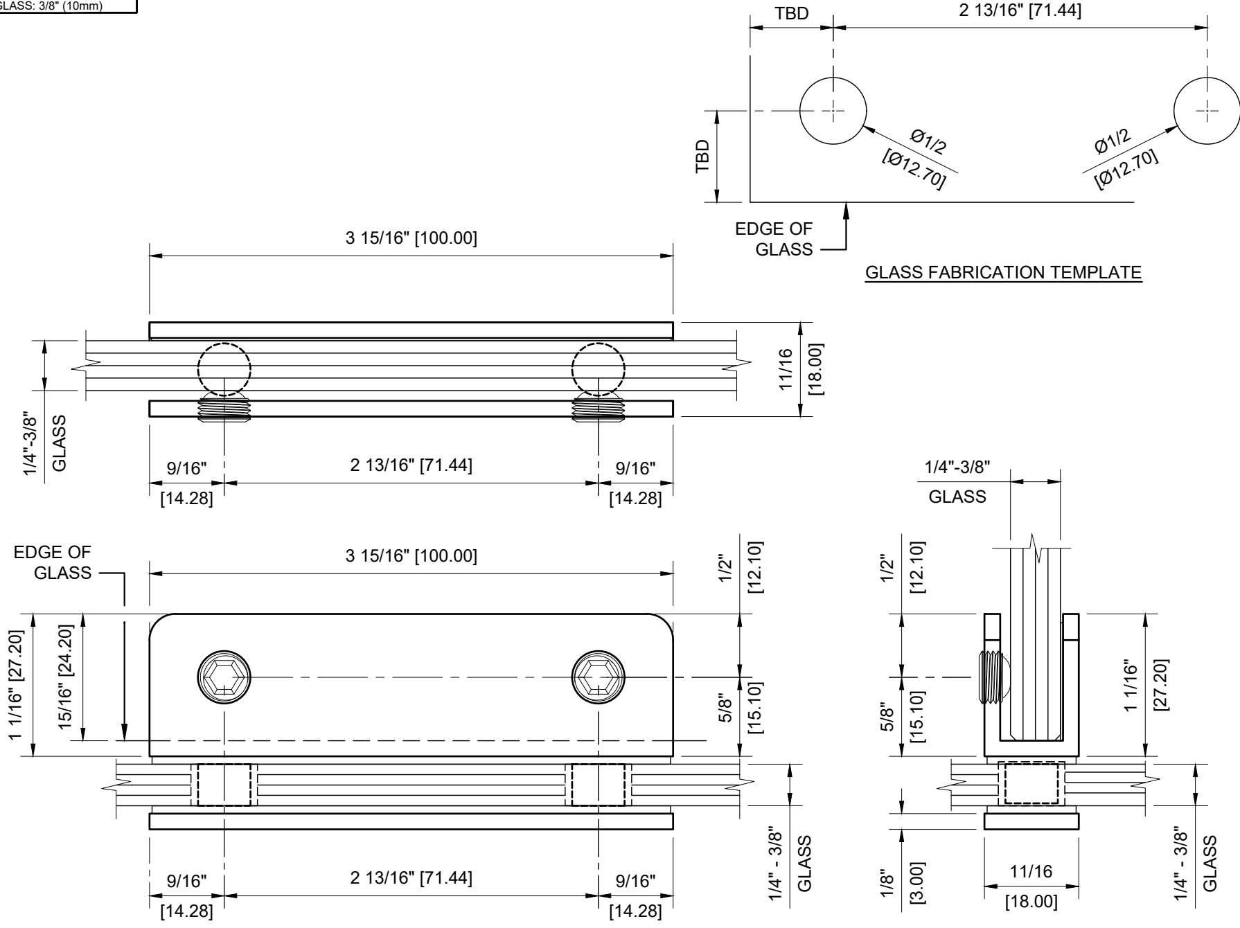
CRL - FA81 THRU GLASS RECTANGULAR SHELF CLAMP FOR 1/4" - 3/8" GLASS
